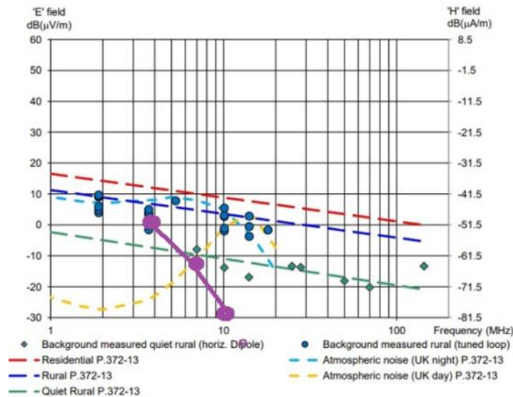
Figure 1 ITU/R P.372-13 expected receiver noise levels together with levels measured by RSGB EMCC 2014 to 2017. REF: https://rsgb.org/main/files/2017/12/221216-Noise-leaflet-issue-2.pdf , page 3
